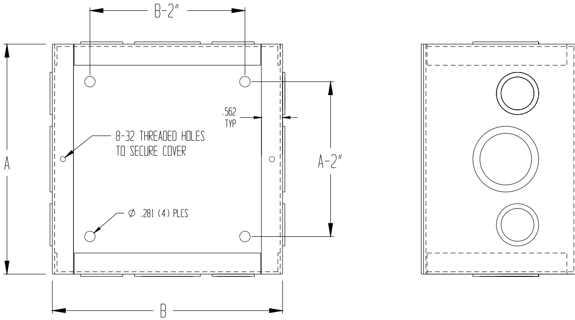
FRONT VIEW (COVER REMOVED)
