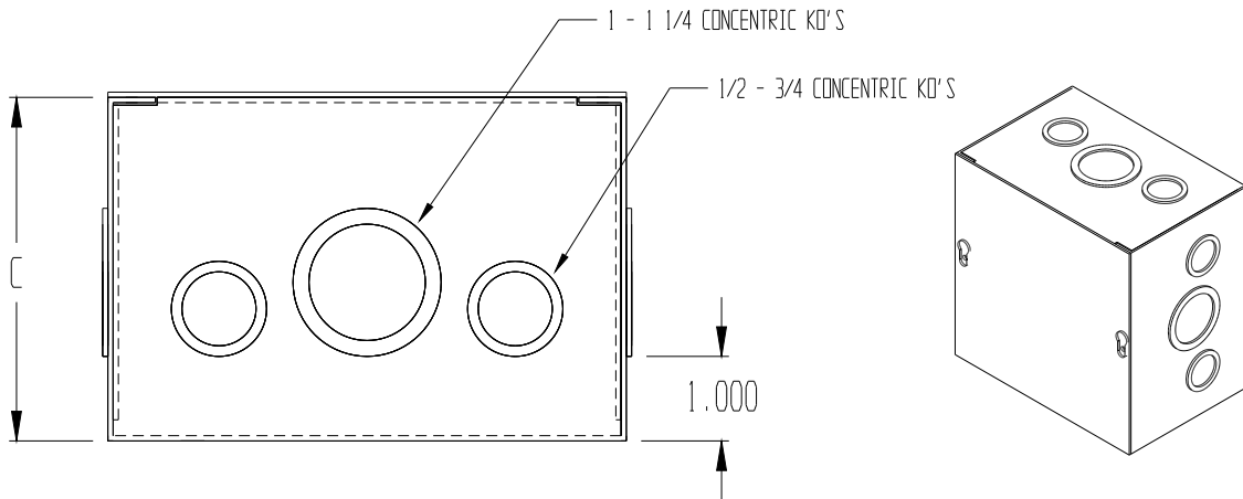
FRONT VIEW (COVER REMOVED)
